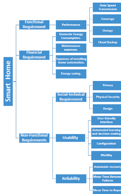
Fig. 2. Users requirements.
