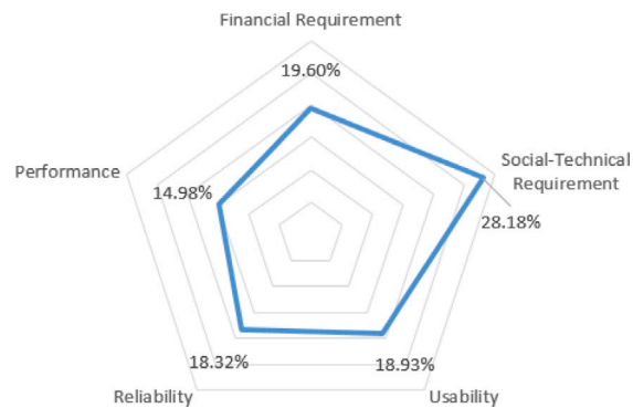
Fig. 4. Requirements ranking.
